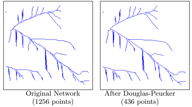
Figure 6: Simplifying the original drainage network using Douglas-Peucker. The refined line network is reduced by a factor of 3 with little visible difference.
