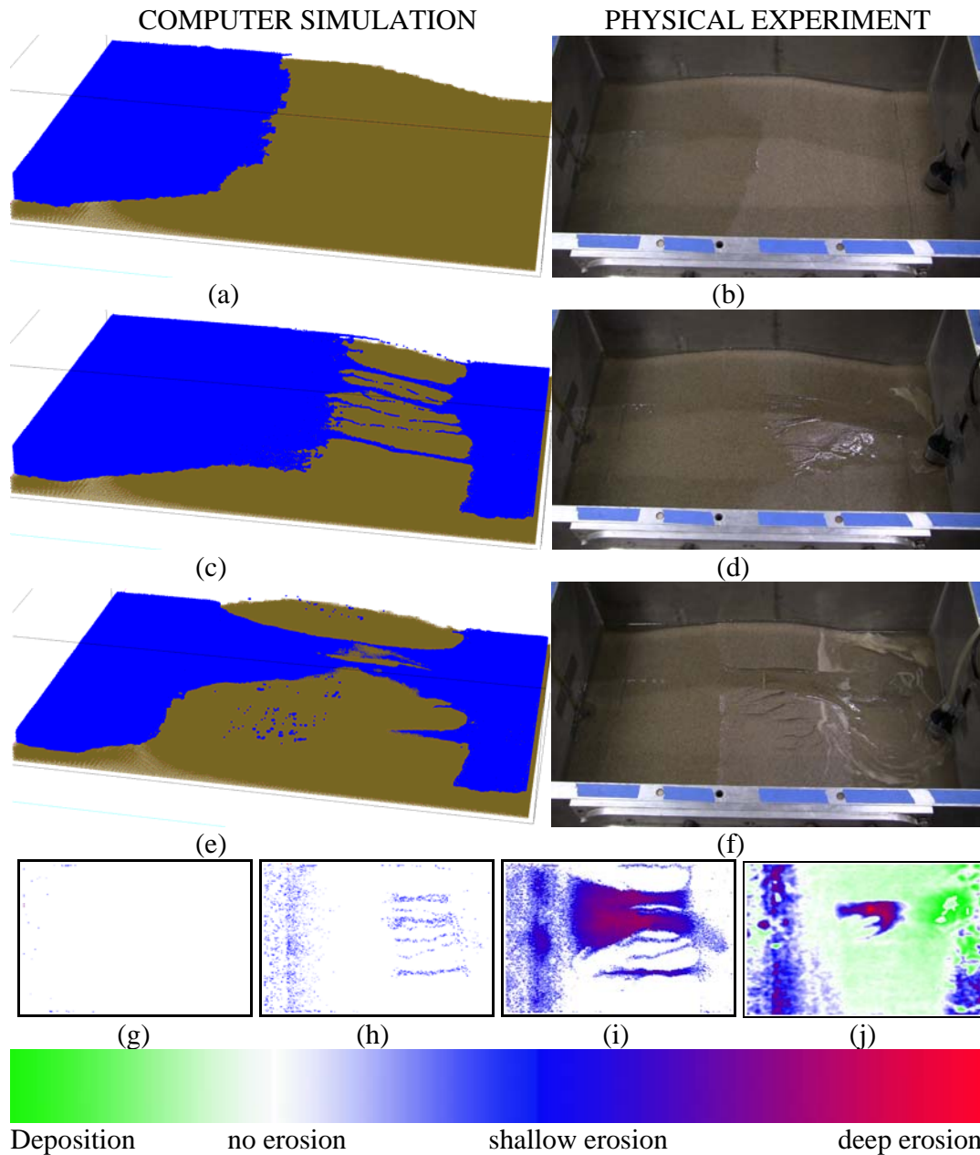
Figure 3. Computer simulation and physical experiment results with pure sand. (a), (c) and (e) are computer simulation results of water and soil represented by particles, while (b), (d) and (f) are physical test results. (a) and (b) were taken at the moment of overtopping. (c) and (d) were taken 1.5 minutes after overtopping. (e) and (f) were taken 10 minutes after overtopping. (g), (h), and (i) visualize the erosion depths corresponding to (a), (c), and (e). (j) shows the depth of erosion
