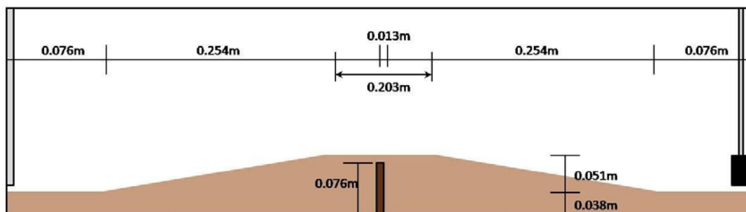
Figure 1. Schematic profile view of physical test setup. The water source is located on the left edge of the diagram, and the sink is on the right edge.
