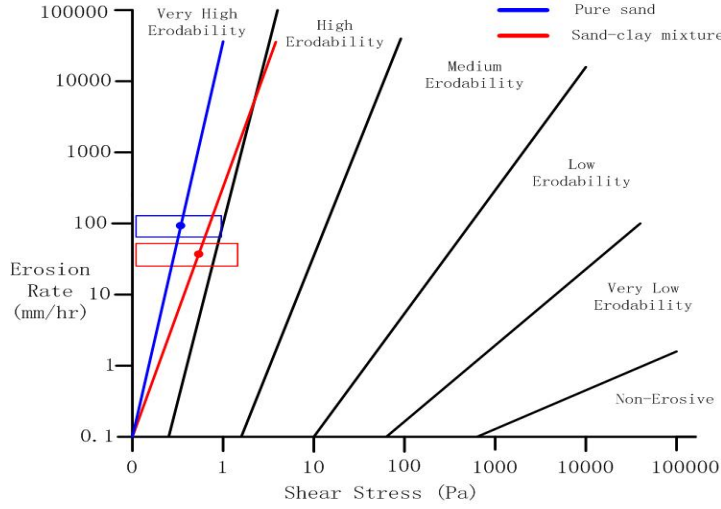
Figure 2. Categories of erodibility and linear erosion functions for materials used in our physical experiments. The boxes of different colors define where the erodibility of the corresponding material lies. The linear erosion function for a single material is calculated by interpolating the origin and a point at the center of the box.
