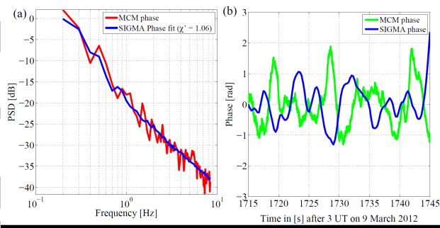
Figure 7. (a) PSD and (b) time series of the best fits for McMurdo with L_{Th} = 40 km thickness at 350 km height.
