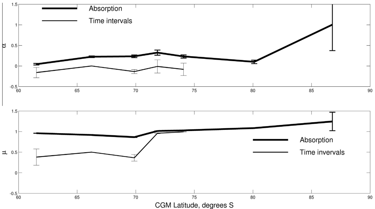
Fig. 6. Latitudinal dependence of power law fitting parameters to (thick line) absorption and (thin line) time intervals time series. (top) \alpha . (bottom) \mu .
