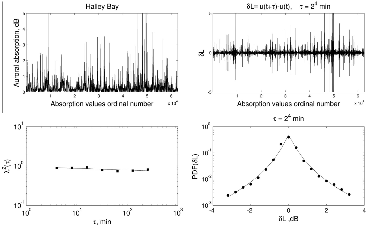
Fig. 5. Sample results of complete analysis. (Clockwise from top left). Observed absorption values, fluctuations, frequency distribution and PDF fitting, power law fitting.
