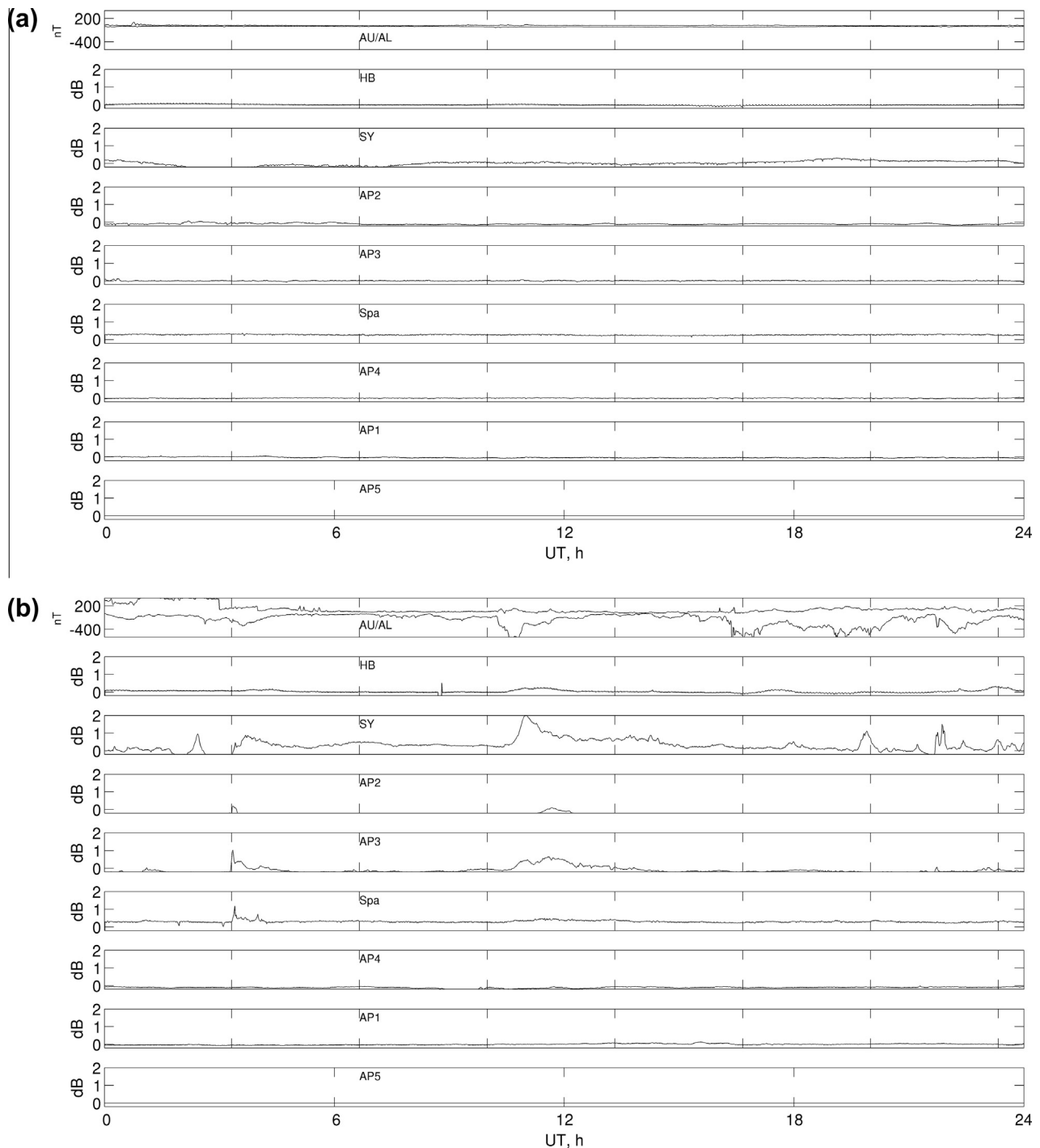
Fig. 3. Sample diurnal variations of riometer auroral absorption at eight Antarctic locations and corresponding AU/AL indices for two days in 1997. (a) Geomagnetic quiet conditions (9 March). (b) Geomagnetic disturbed conditions (27 January).
